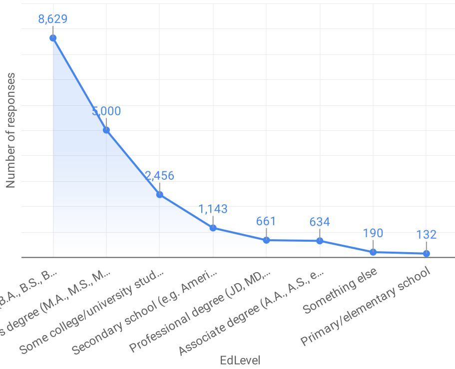
Respondent Distribution by Education Level
