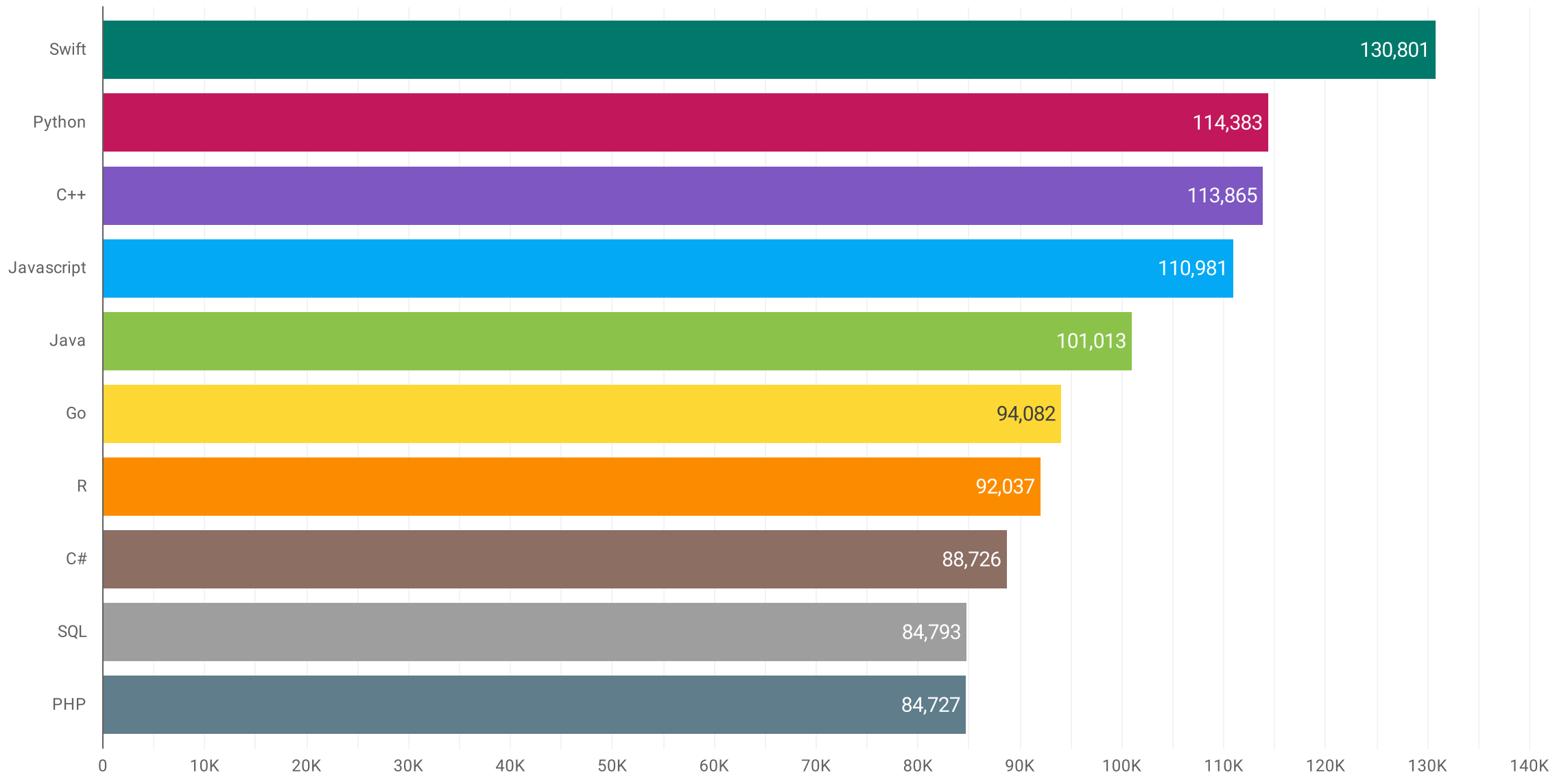
Average Salary by Language Name
